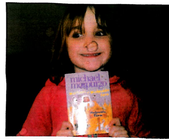
Rectangle ✓
