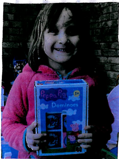
Cuboid ✓
